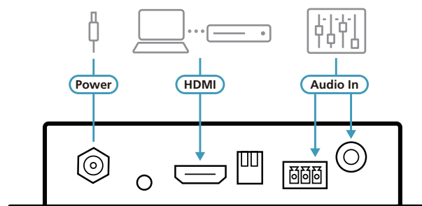
Rear View
